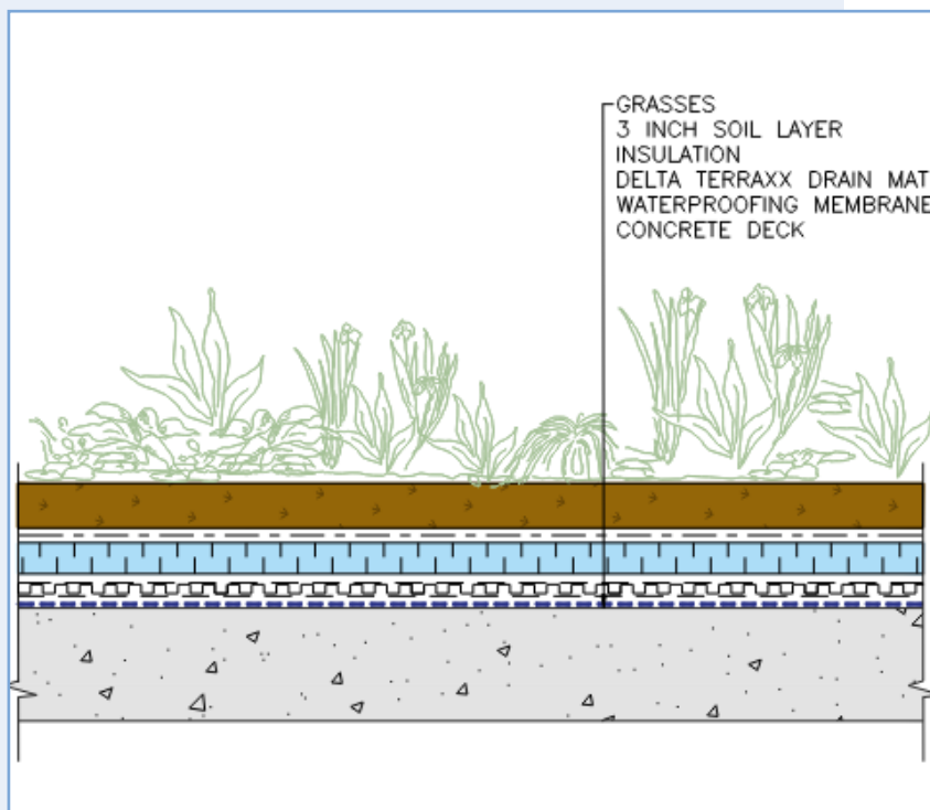
FIGURE 4: Green Roof – Unoccupied – Extensive
